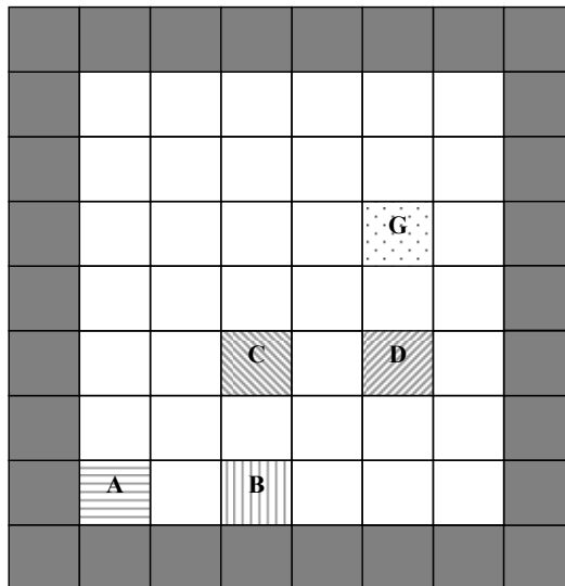
Fig. 2. The cellular environment that is similar to the “world” in Fig. 1, but the landmarks A, B, C, D, G are separated by one cell distance
