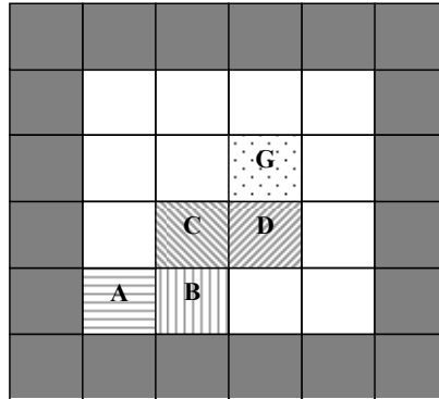
Fig. 1. Simple cellular environment. The landmarks A, B, C, D, G are in adjacent cells. The cell G is the goal cell. The “world” consists of 4x4 cells; it is surrounded by impenetrable barriers (grey cells)
